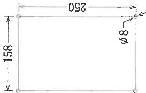
Installation size
